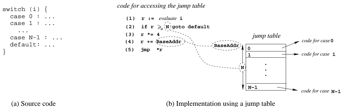
Figure 3: A example of a C switch statement and its implementation using a jump table
