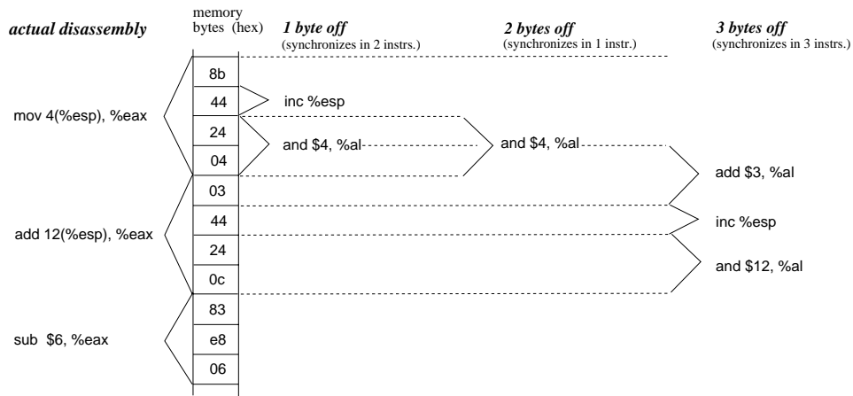
Figure 4: An example of self-repairing disassembly
