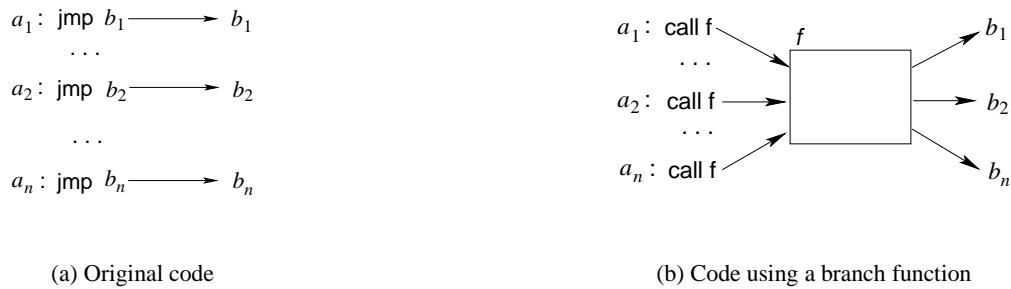
Figure 5: Branch functions
