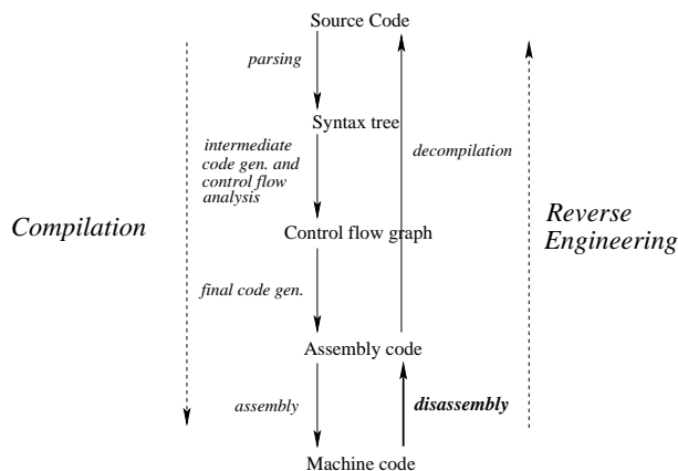
Figure 1: The processes of compilation and reverse engineering
