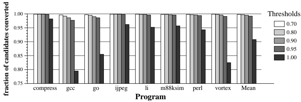
(a) Fraction of jumps converted to branch function calls
