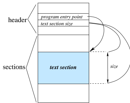
Figure 2: The structure of an executable file
