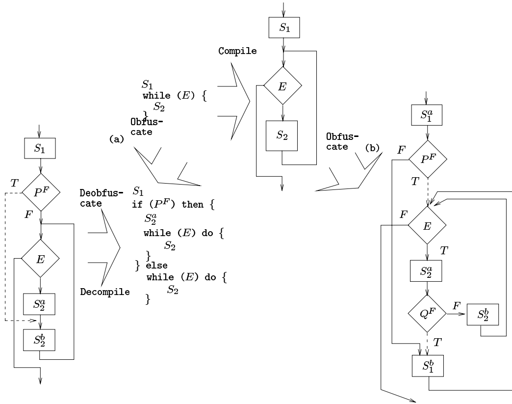
Figure 12: Reducible to Non-Reducible Flow graphs. In (a) we split the loop body S_2 into two parts ( S_2^g and S_2^b ), and insert a bogus jump to the beginning of S_2^g . In (b) we also break S_1 into two parts, S_1^a and S_1^b . S_1^b is moved into the loop and an opaque predicate P^F ensures that S_1^a is always executed before the loop body. A second predicate Q^F ensures that S_1^b is only executed once.
