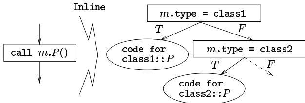
Figure 14: Inlining method calls. Unless we can statically determine the type of m , all possible methods to which \overline{m.P()} could be bound must be inlined at the call site.
