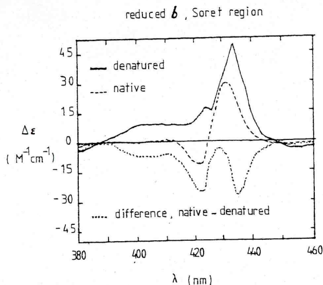
Fig. 2. Resolved CD spectra of the b cytochromes in the Soret region. The reductase was suspended at 6.6 \mu\text{M} cytochrome b in the Tris-glycerol-cholate buffer (6) and reduced with dithionite. The CD spectrum of reduced xanthine oxidase adjusted to the same signal at 470 nm was subtracted from that of native reduced fumarate reductase. This was done to correct for the interfering spectrum of the 2Fe-2S cluster. The denatured enzyme was obtained as in Fig. 1 and its optical spectrum (not shown) was very similar to that of the native enzyme in the Soret region, and 1 nm blue-shifted in the \alpha region.
